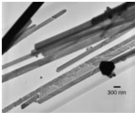
Figure 3. TEM micrograph of indium nanowires prepared in the presence of HDA (0.5 equiv).
